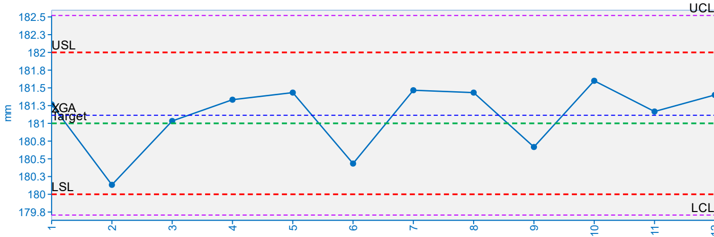
X-Bar Chart
