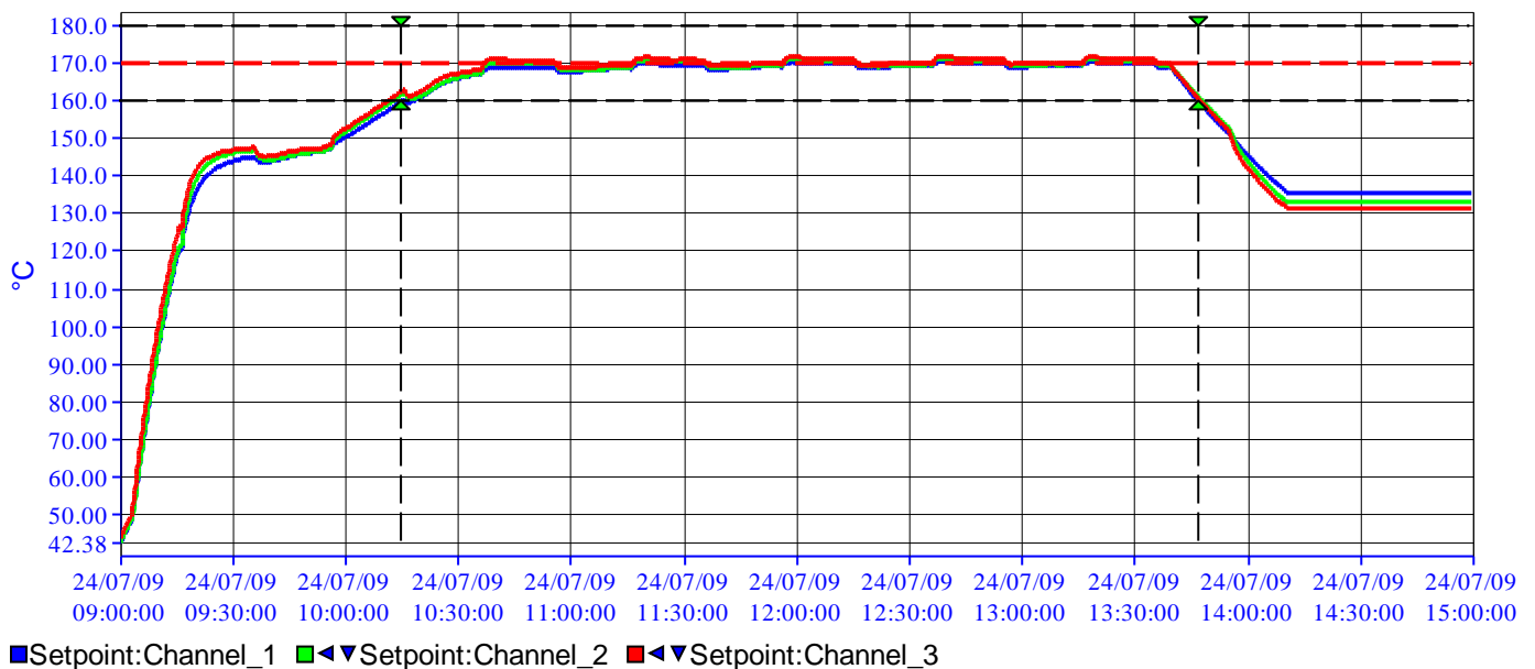
Process Chart
